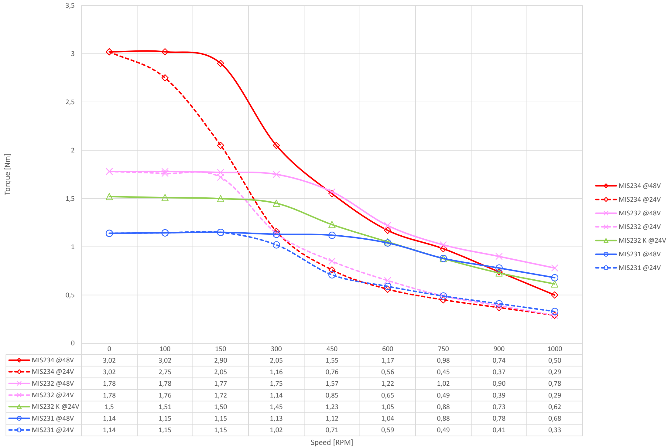
MIS23x Torque vs Speed curve
