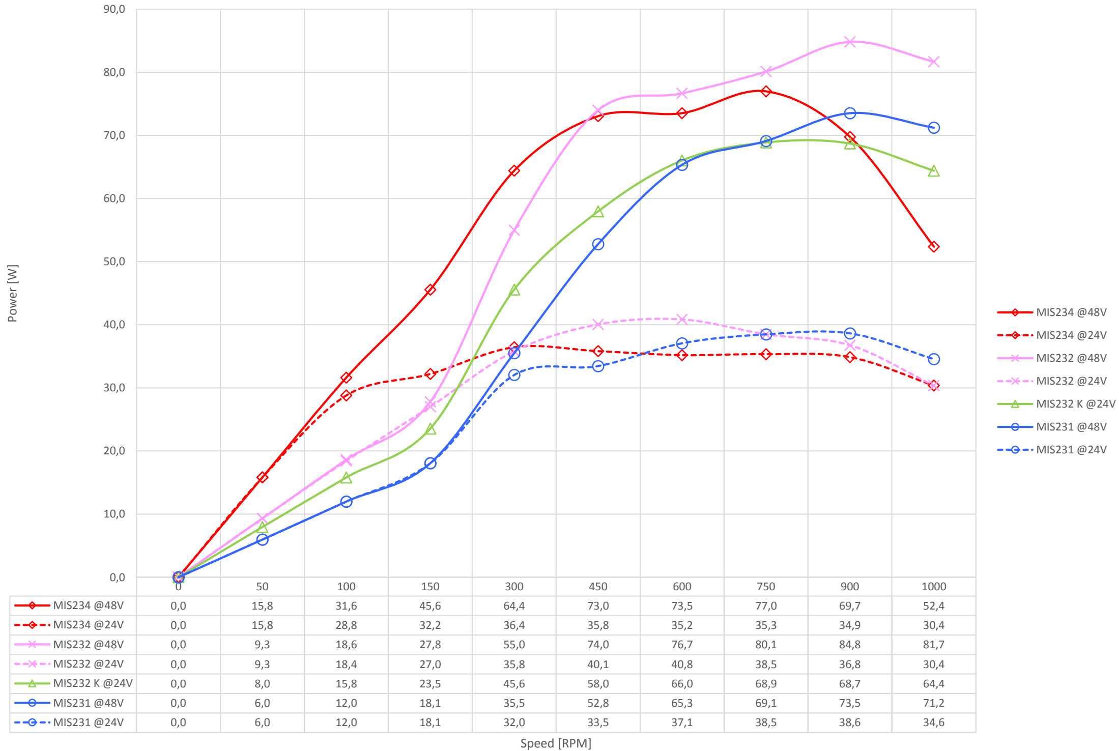
MIS23x Power vs Speed curve
