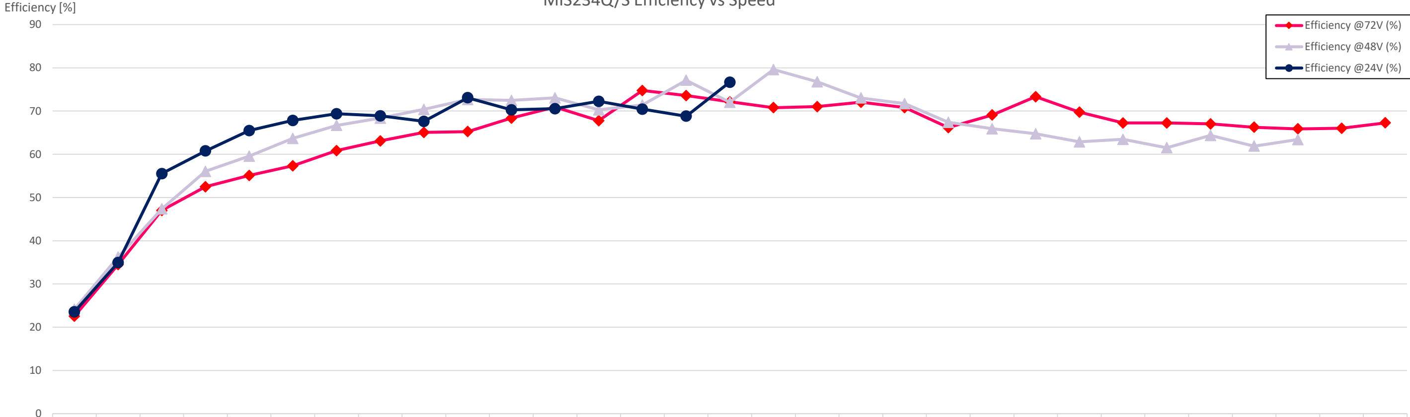
MIS234Q/S Efficiency vs Speed
