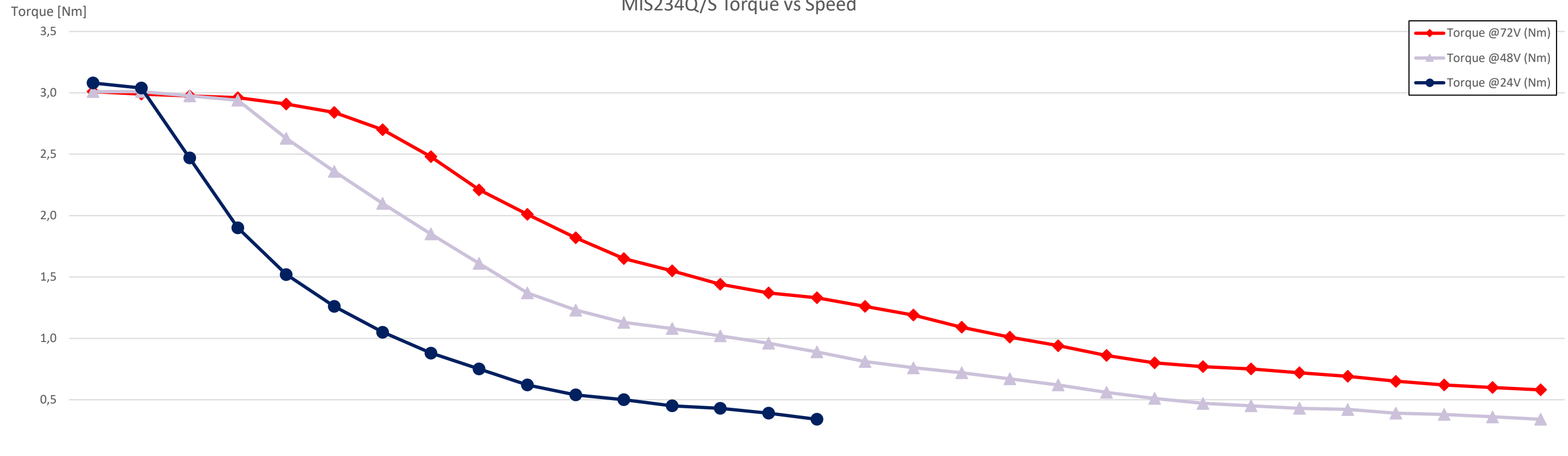
MIS234Q/S Torque vs Speed
