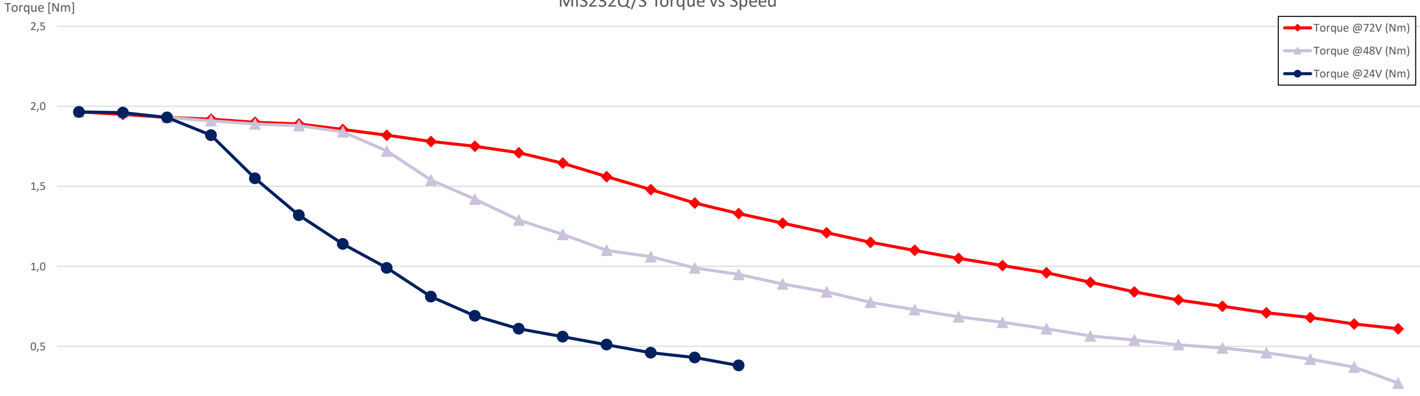
MIS232Q/S Torque vs Speed
