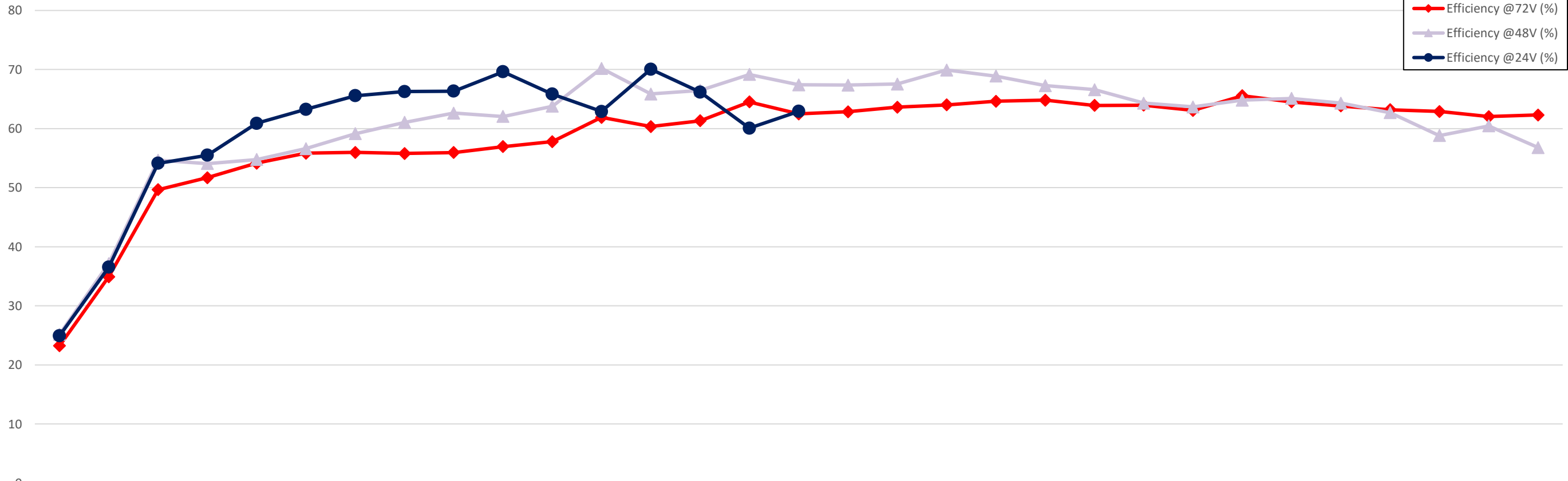
MIS232Q/S Efficiency vs Speed
