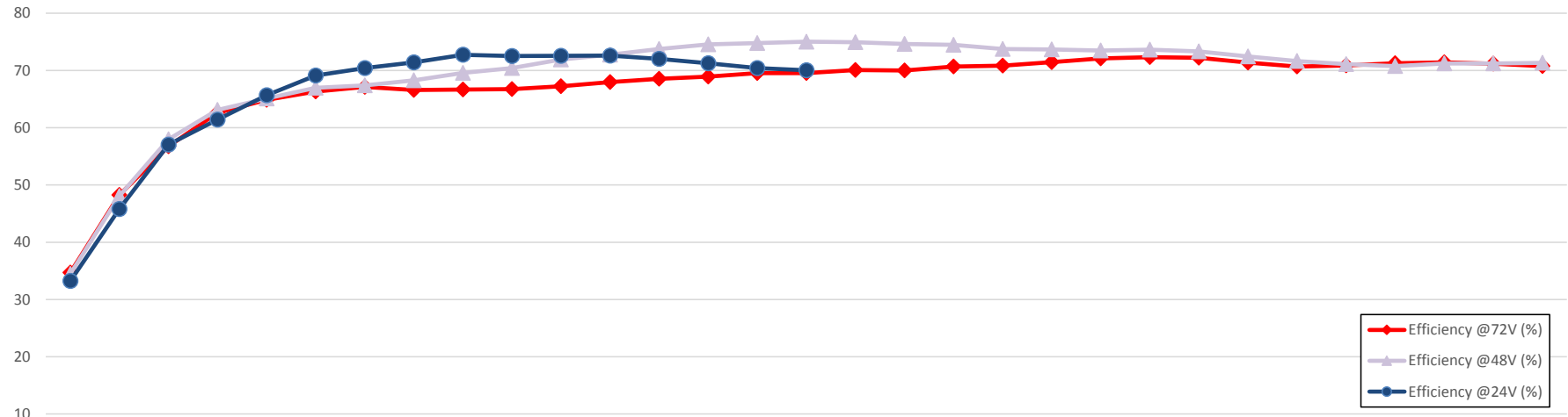
MIS232T Efficiency vs Speed
