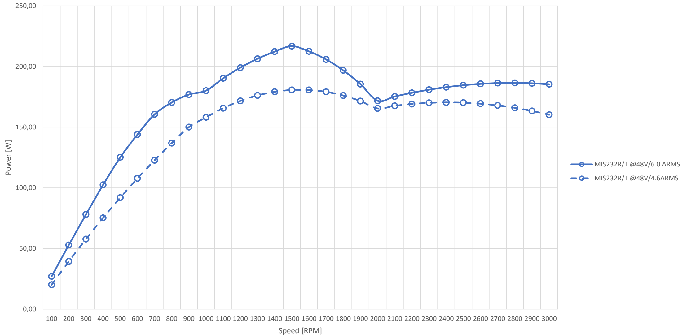
MIS232R/T Power vs Speed Curve
