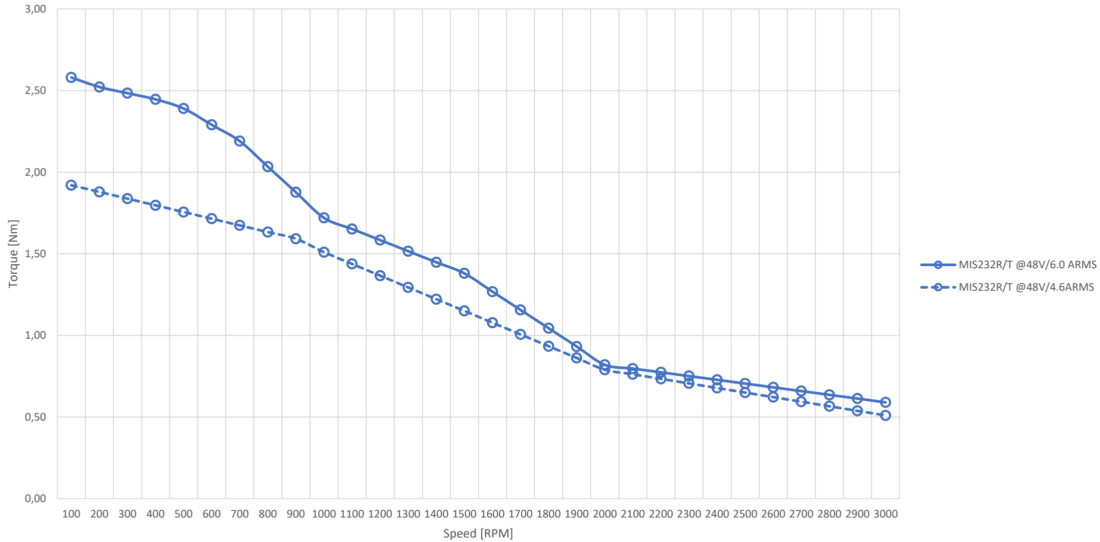
MIS232R/T Torque vs Speed Curve
