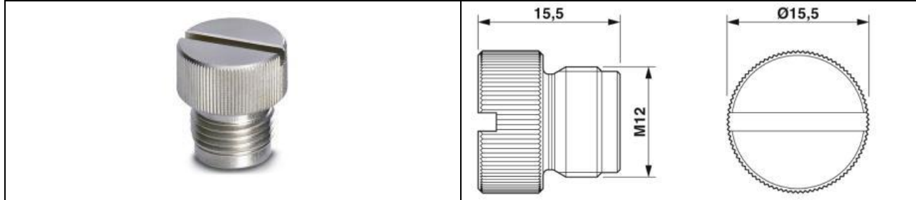
WI1000-M12FCAP2 (fit on female connector)
