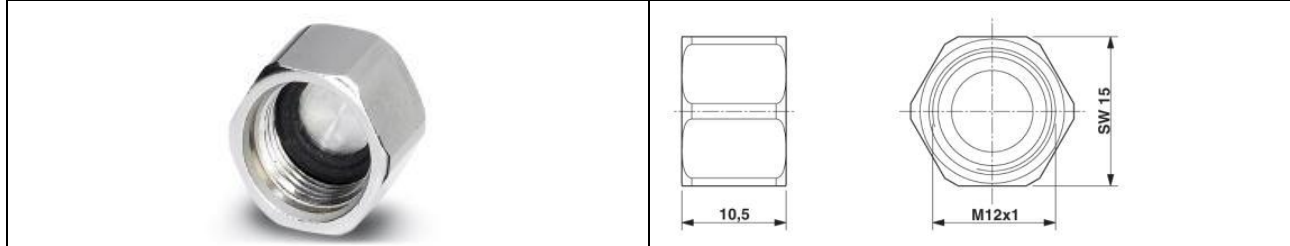
WI1000-M12FCAP2 (fit on female connector)
